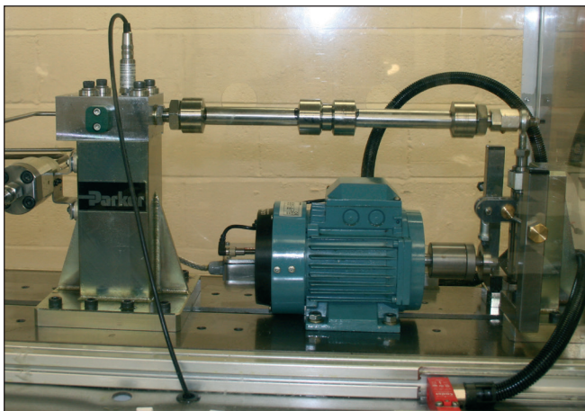
Flexural test
